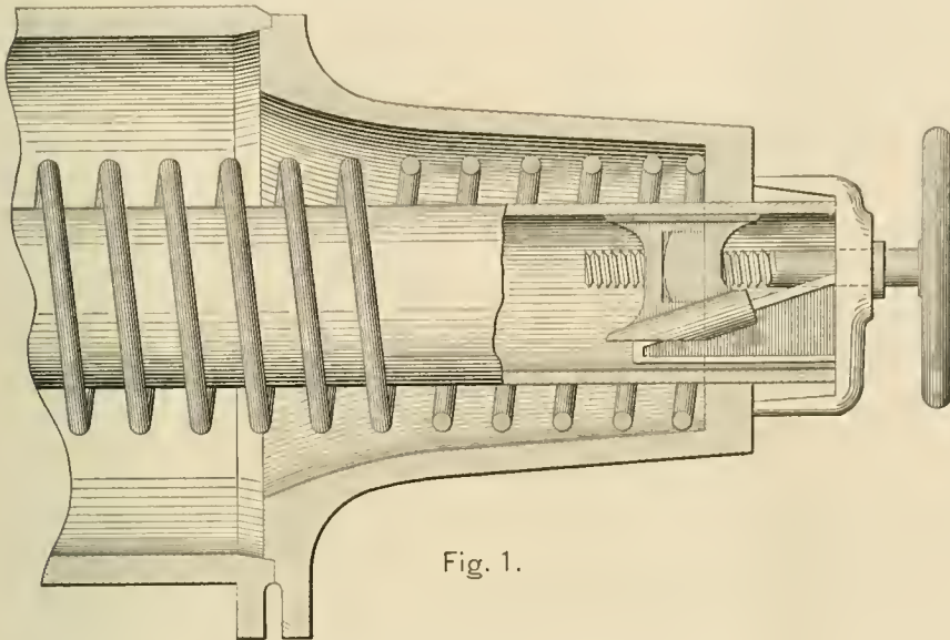
DEVICE FOR HOLDING PARTS INTACT WHILE CLEANING. SCREW DRAWS NUT UP INCLINE, FORCING OUTWARD ON INNER SIDE OF PISTON SLEEVE.
